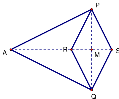
Figure 2.6: Peaucellier's linkage.
