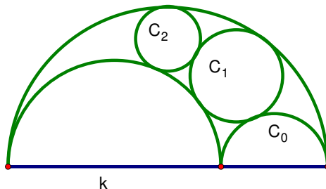
Figure 2.2: The shoemaker's knife.
