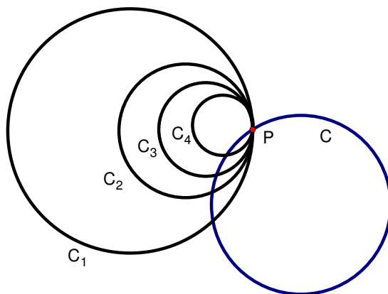
Figure 2.1: Four circles are internally tangent at P , with a fifth circle passing through P .
