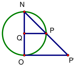
Figure 3.3: OP' \parallel QP , so that \triangle NQP and \triangle NOP' are similar.
