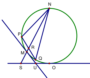
Figure 3.5: A cross-section of the sphere.
